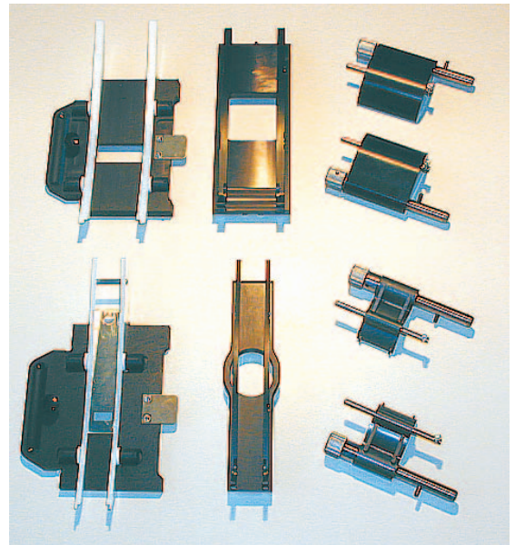
Replacement parts for change of format: on the top: 70 mm / at the bottom: 35 mm
